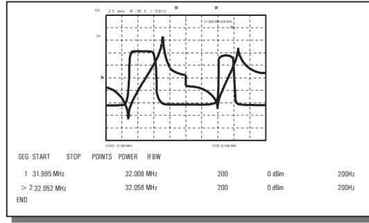
Example of crystal resonator measurement
