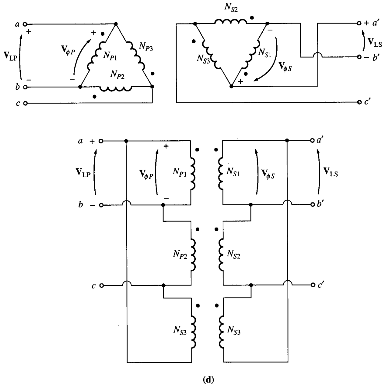
FIGURE 2-38 Three-phase transformer connections and wiring diagrams: (d) \Delta - \Delta (concluded)
