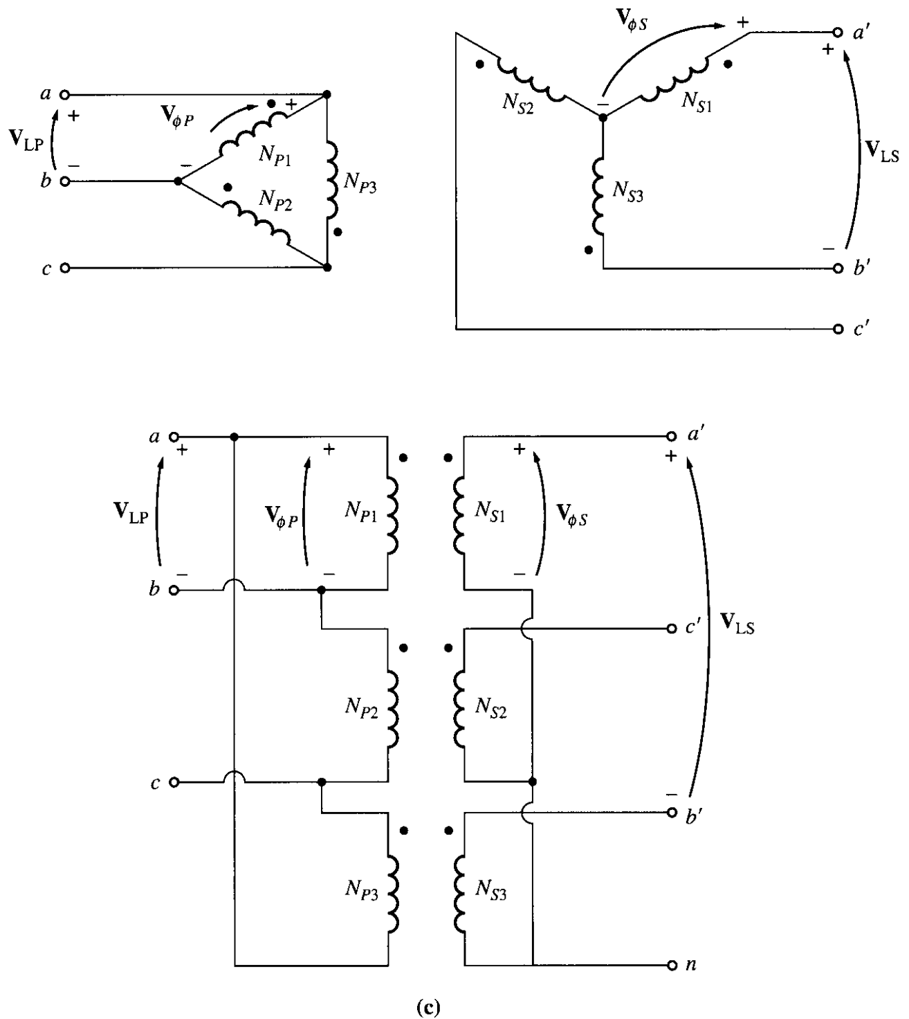
FIGURE 2-38 Three-phase transformer connections and wiring diagrams: (c) \Delta -Y ( continued )
