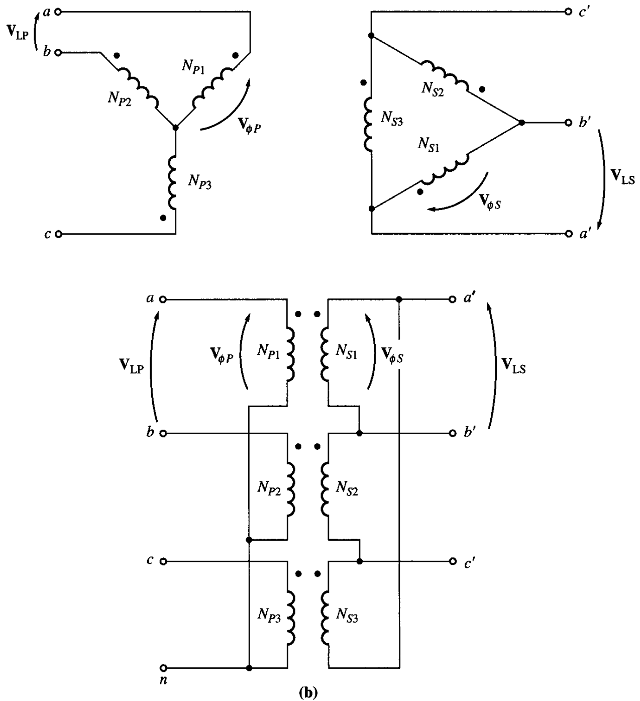
FIGURE 2–38 Three-phase transformer connections and wiring diagrams: (b) Y–Δ ( continued )
