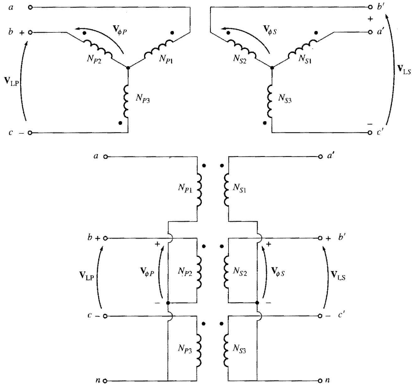
Figure 3-37 | Three-phase transformer connections and wiring diagrams:
