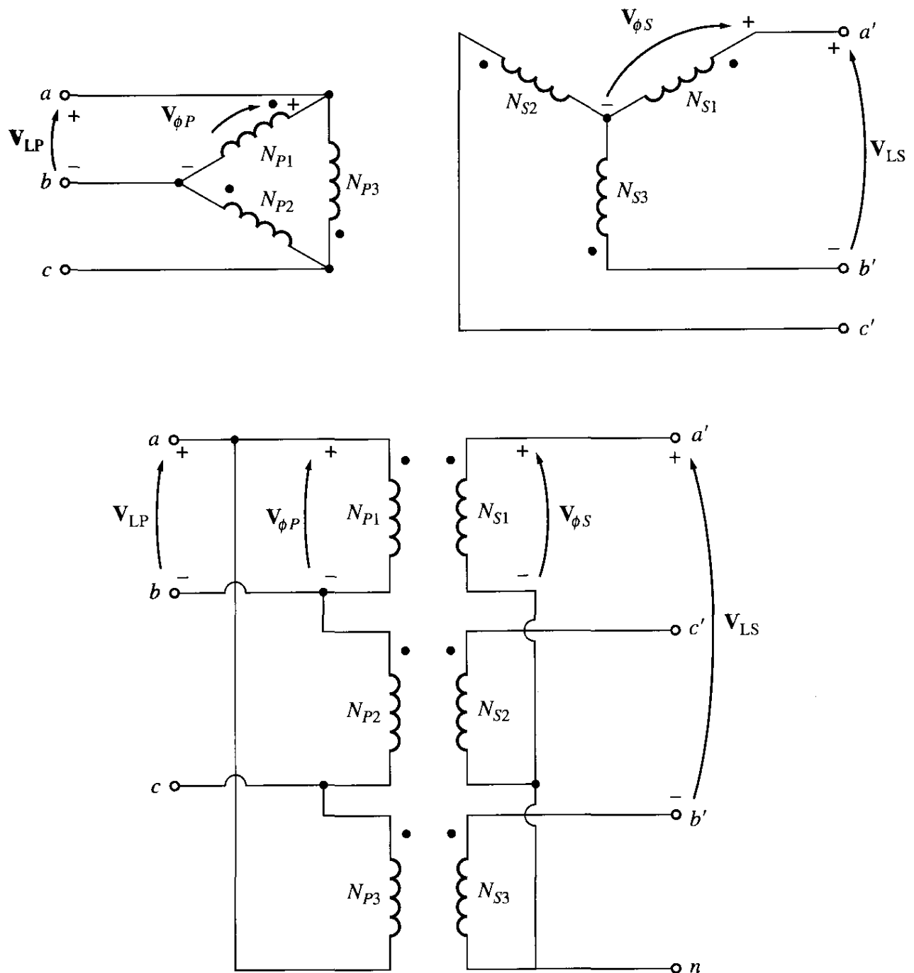
(c) \Delta -Y (continued)
