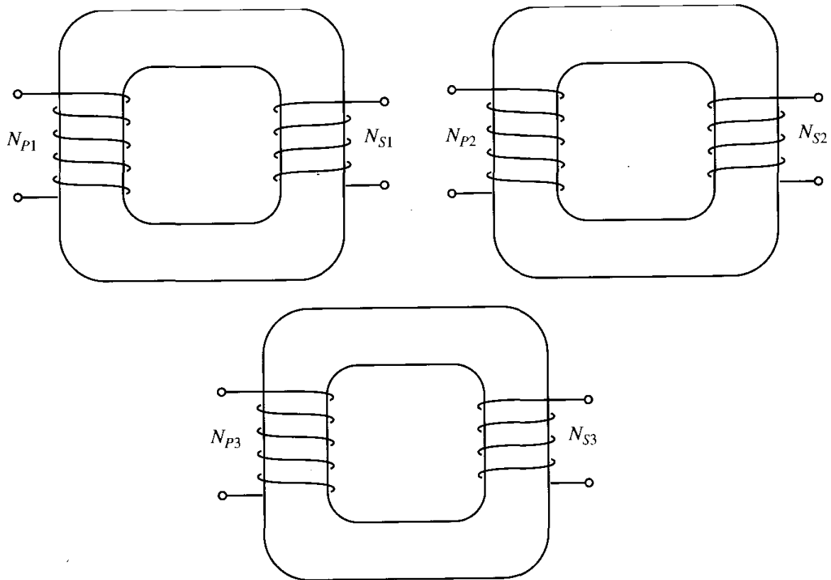
Figure 3–35 | A three-phase transformer bank composed of independent transformers.
